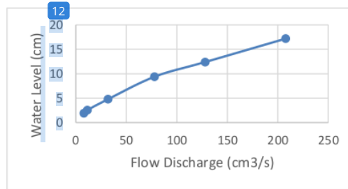
Fig. 5. Graph of Relationship between Water Level and Discharge Before Leap
